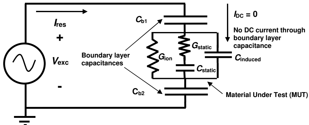
Figure 30-15 Circuit model of polymer with boundary layer capacitances
