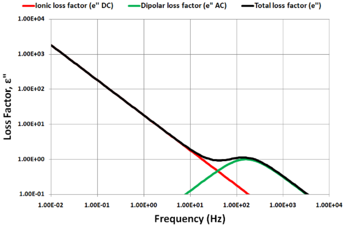
Figure 30-12b Effect of intermediate conductivity on loss factor (modeled)
