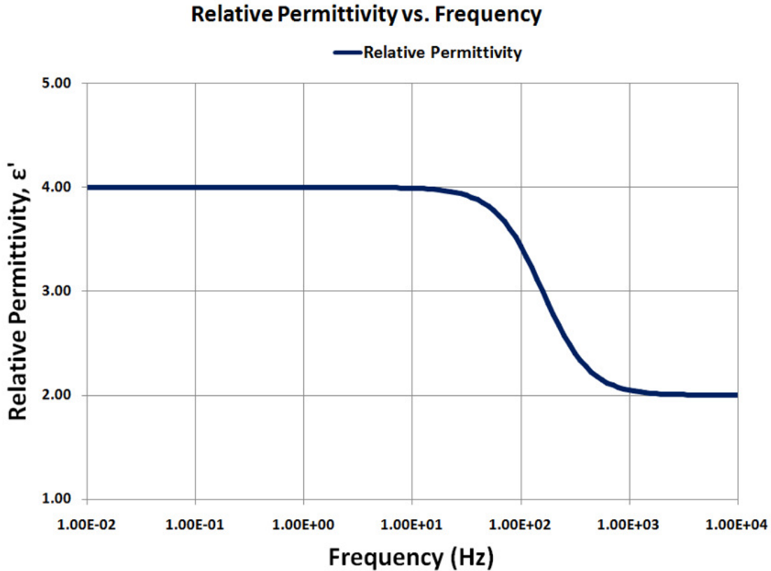
Figure 30-13 Ideal frequency response of relative permittivity (Corresponding to example modeled in Figure 30-12)
