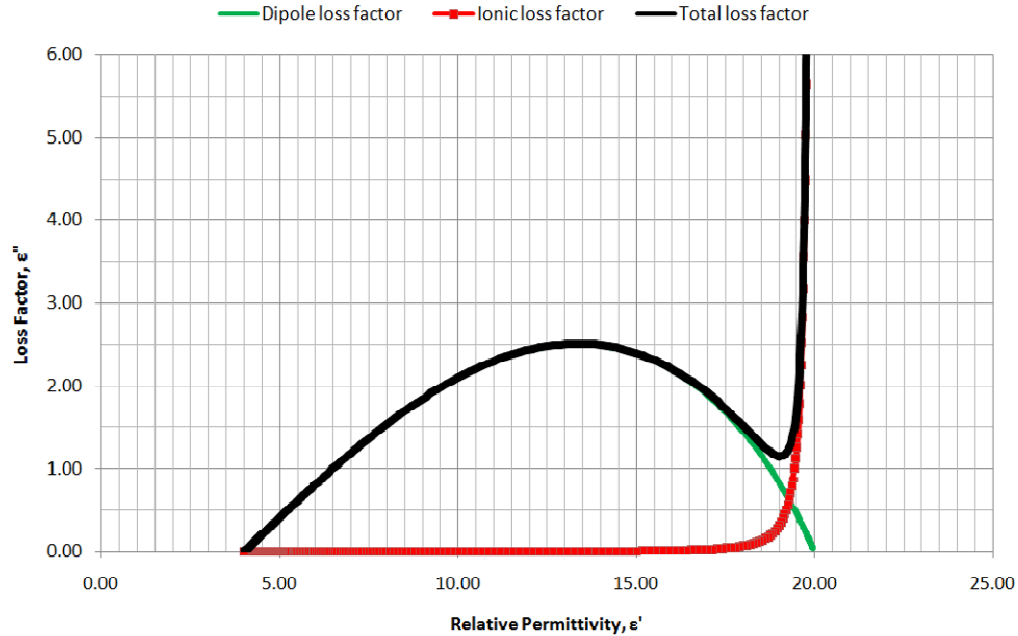
Figure 30-10 Addition of ionic and dipolar loss factors
