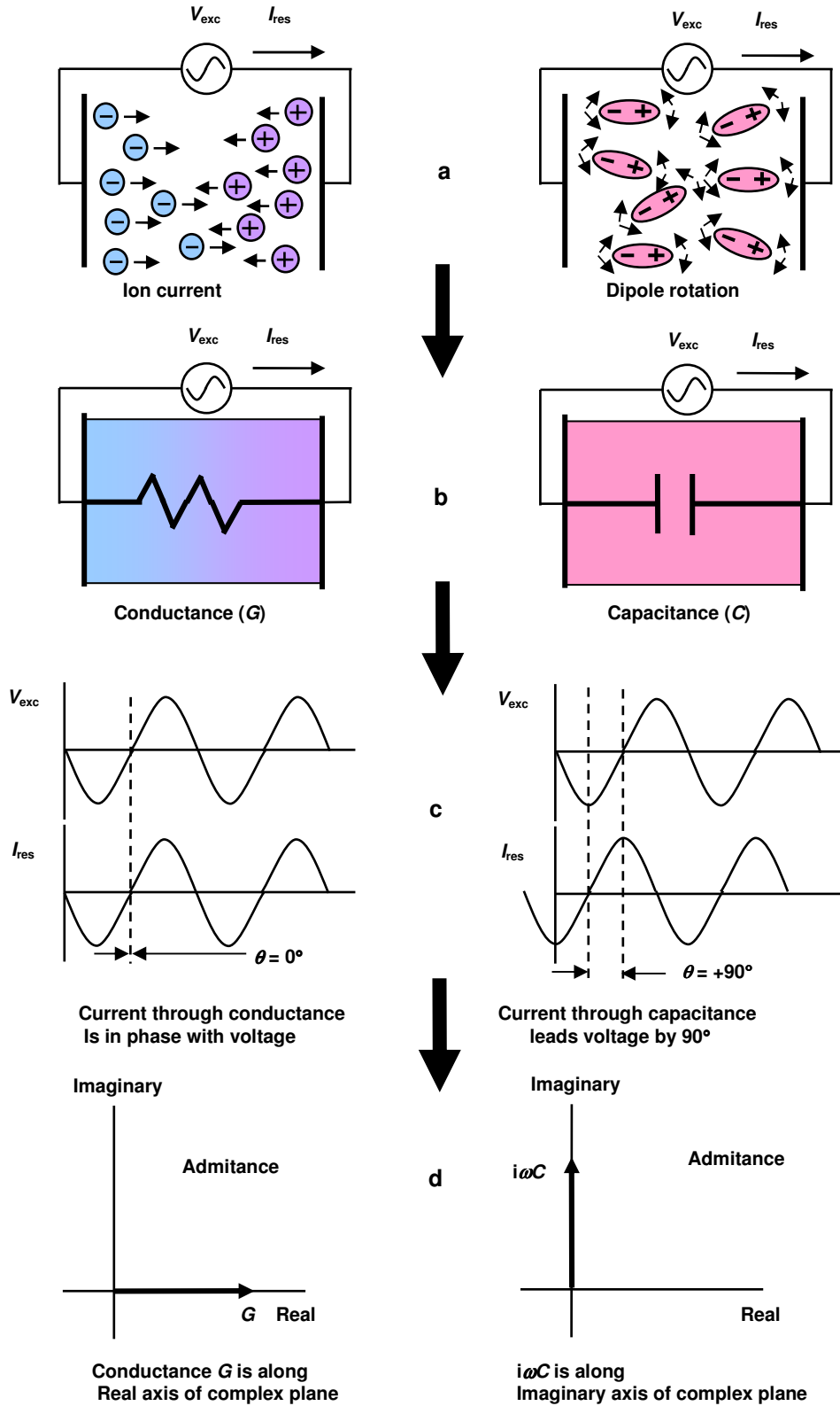
Figure 30-1 Relationships between physical and electrical behavior
