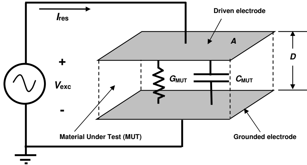
Figure 30-3 Electrical model of a polymer
