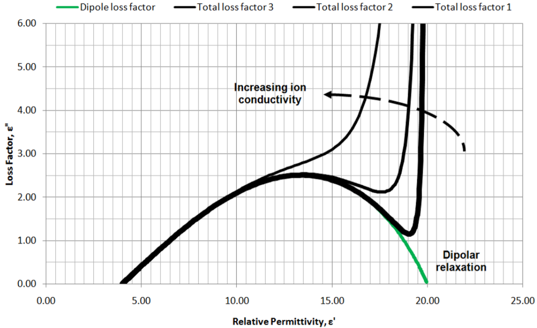
Figure 30-11 Total loss factor as a function of increasing ionic conductivity
