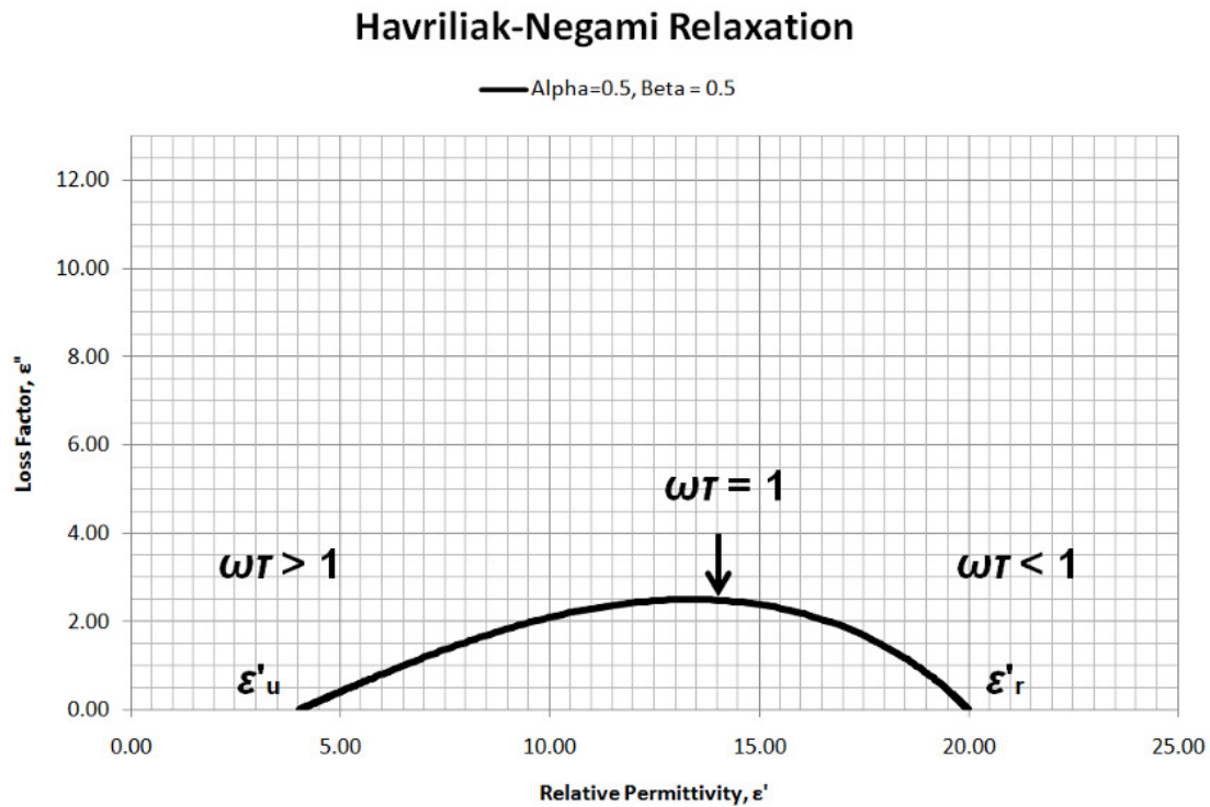
Figure 30-9 Cole-Cole plot of Havriliak-Negami relaxation
