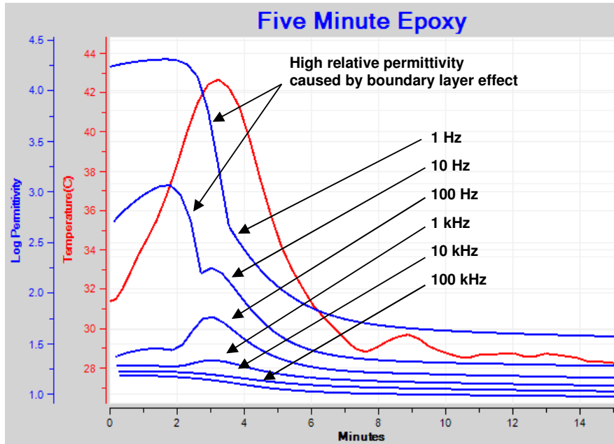
Figure 30-21 Relative permittivity of curing epoxy, showing effect of boundary layer
