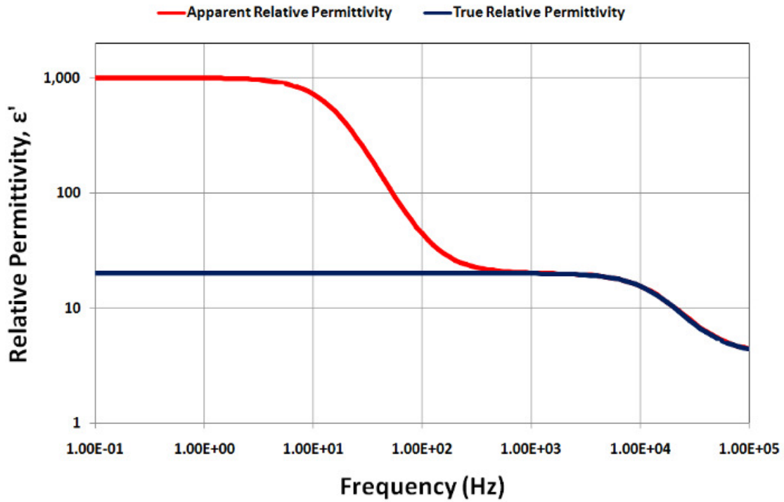
Figure 30-19a ε' with electrode polarization and small dipole time constant
