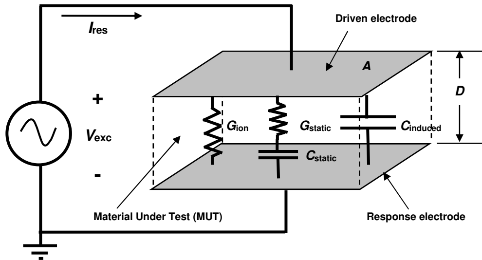
Figure 30-4 Electrical model of polymer physical behavior
