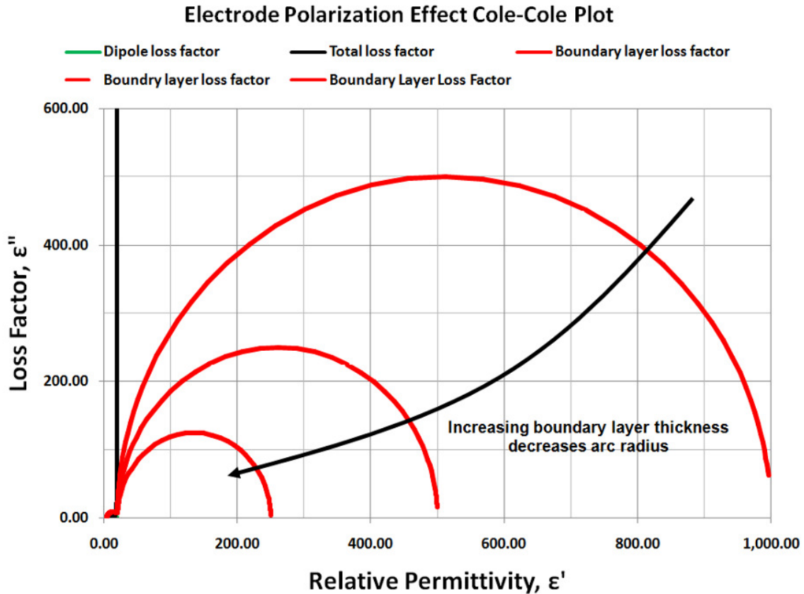
Figure 30-18 Cole-Cole plot trajectories caused by electrode polarization
