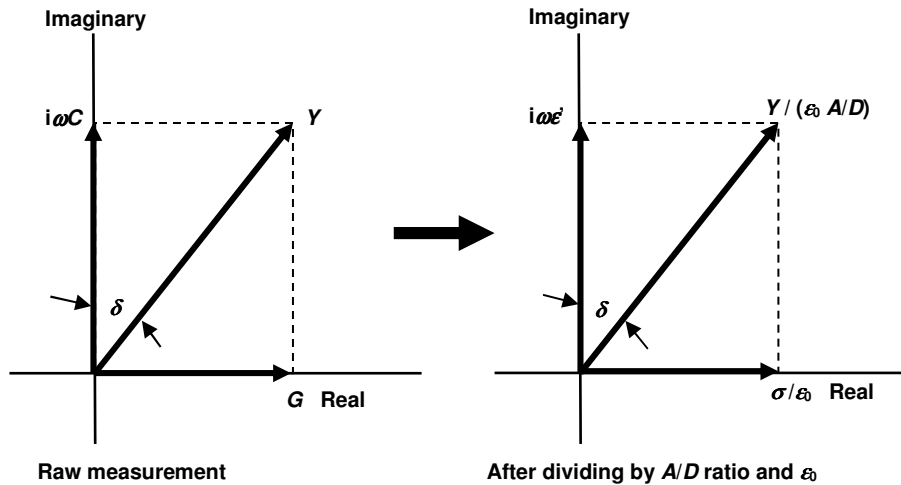
Figure 30-2 Relationship between bulk and material properties
