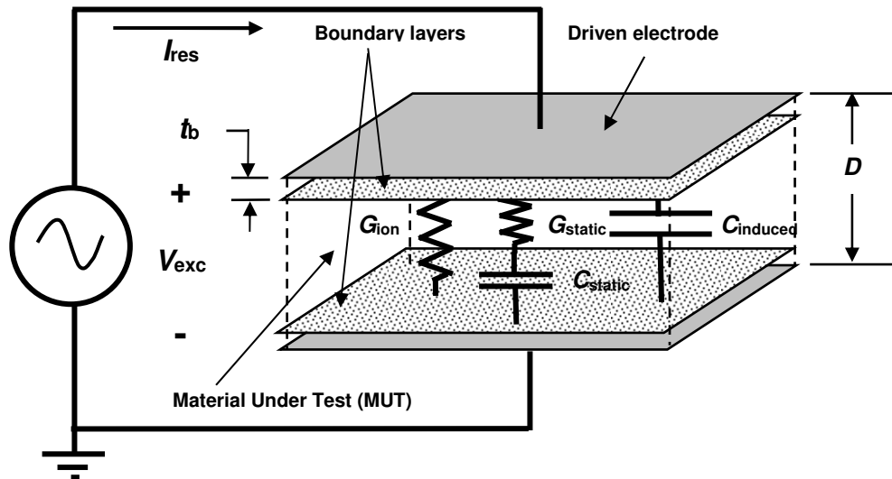
Figure 30-14 Boundary layer capacitances resulting from electrode polarization
