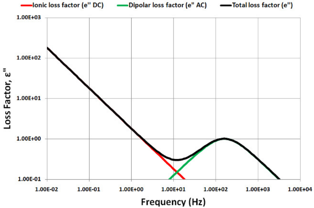
Figure 30-12a Effect of low conductivity on loss factor (modeled)
