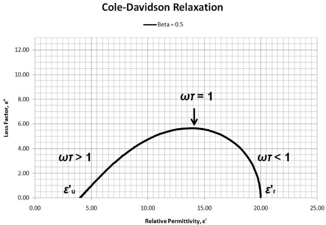
Figure 30-8 Cole-Cole plot of Cole-Davidson relaxation
