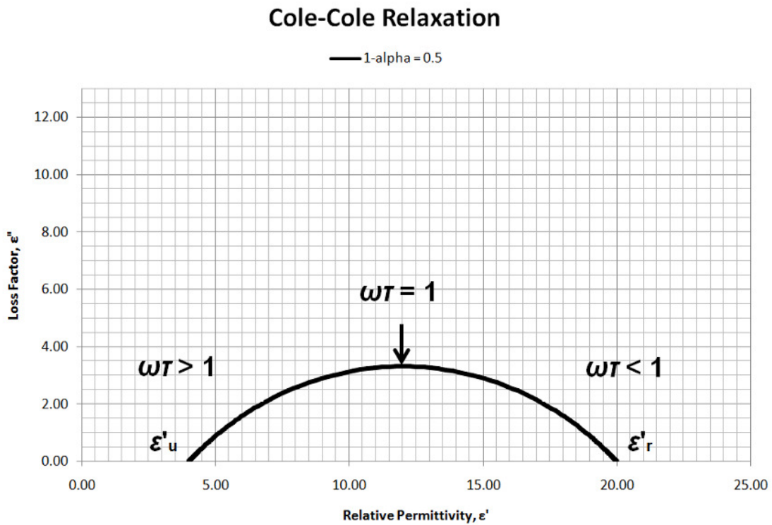
Figure 30-7 Cole-Cole plot of Cole-Cole relaxation
