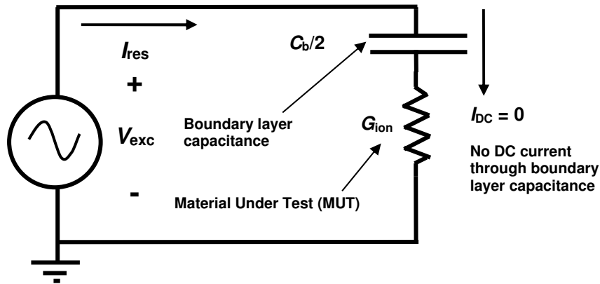
Figure 30-16 Low frequency circuit model with boundary layer capacitance
