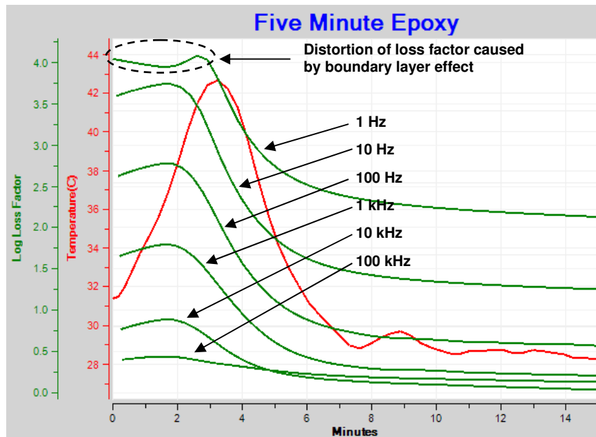
Figure 30-22 Loss factor of curing epoxy, showing effect of boundary layer
