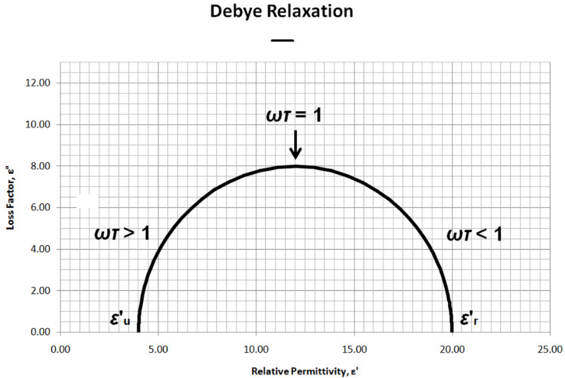
Figure 30-6 Cole-Cole plot of Debye relaxation
