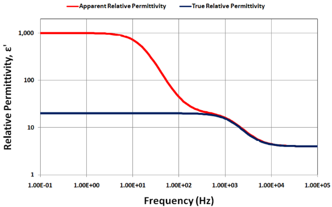
Figure 30-19b ε' with electrode polarization and intermediate dipole time constant
