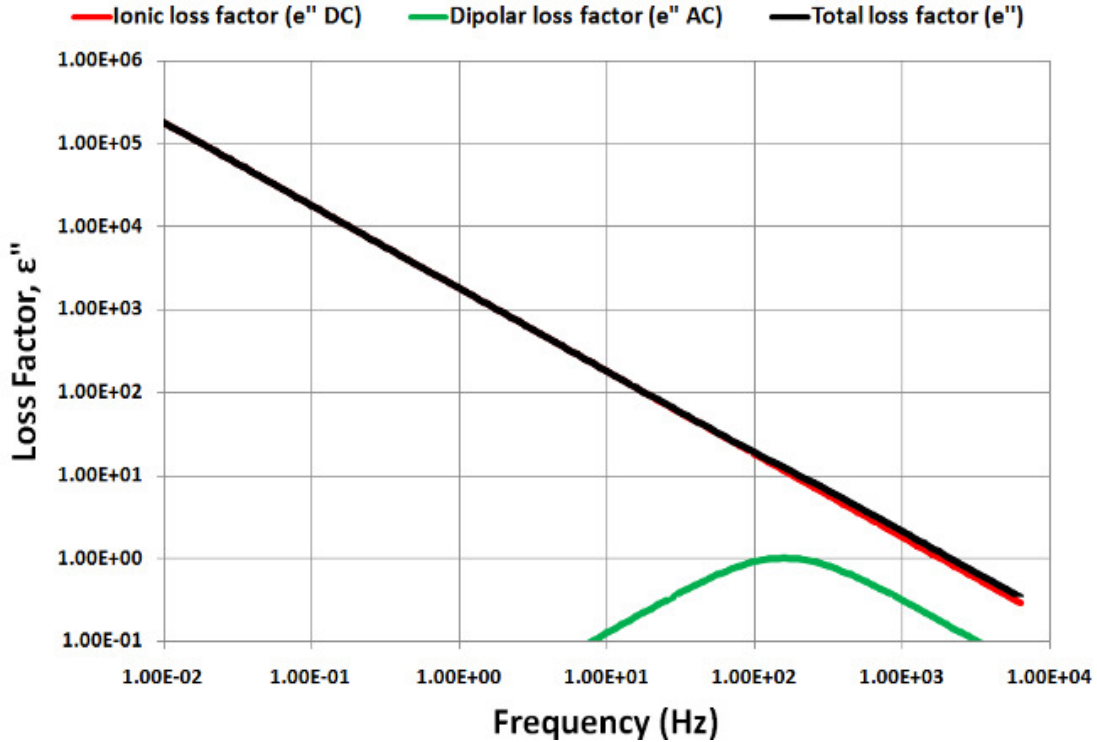
Figure 30-12 Effect of high conductivity on loss factor (modeled)
