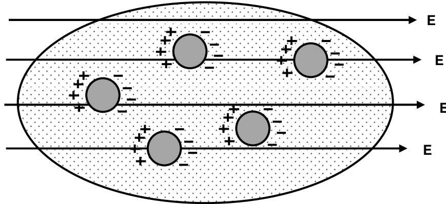
Figure 30-23 Maxwell-Wagner-Sillars polarization
